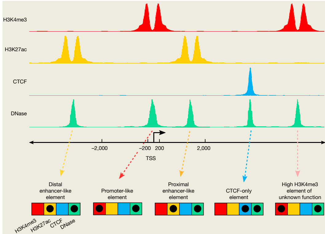
Box 1 Fig. 1 | Classification of cCREs by epigenetic signatures and proximity to TSS.
