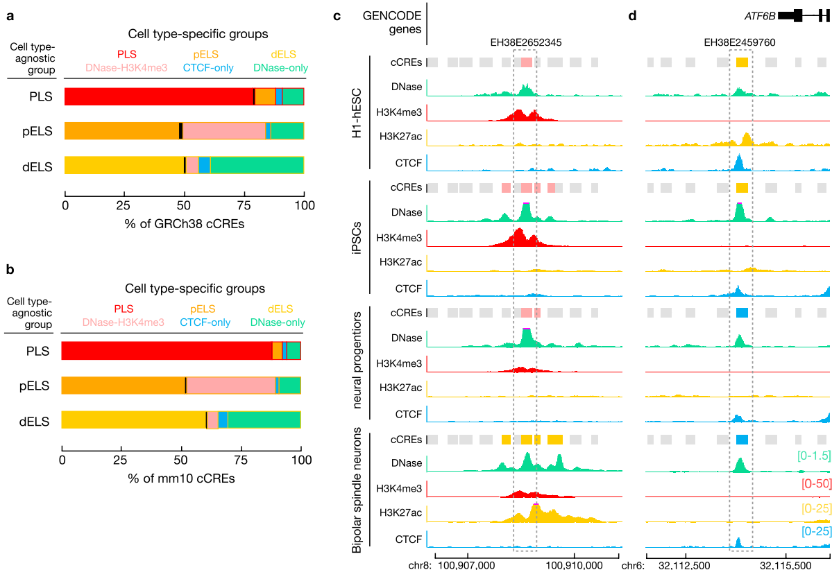
Extended Data Fig. 1 | Classification of human cCREs is largely consistent across biosamples. a, b , For the 25 human (a) and 15 mouse (b) biosamples that were covered by all four core assays, we analysed how cCRE classification could differ between biosamples. For each cell-type-agnostic group of cCREs, the bars indicate their group classification in specific biosamples, coloured by group as indicated. Black indicates a switch in the grouping, for example, from cell type-agnostic PLS to cell type-specific pELS or CTCF-only. c, d , Two example switches of cCRE grouping between different biosamples. c , EH38E2652345 is a cCRE-dELS that has high DNase, H3K4me3, and H3K27ac signals in bipolar spindle neurons. By contrast, in cell types at earlier stages of
