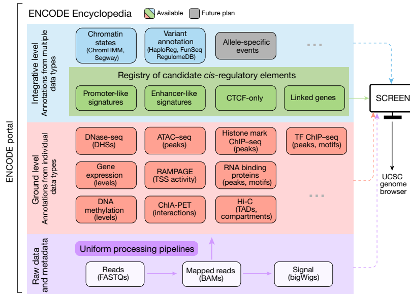
Fig. 2 | Overview of the ENCODE Encyclopedia with a registry of candidate cis-regulatory elements. The ENCODE Encyclopedia consists of ground-level and integrative-level annotations that use data processed by the uniform
