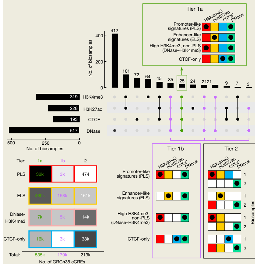
Box 1 Fig. 2 | Profiles of feature ascertainment across biosamples and confidence tiers for cCREs.
