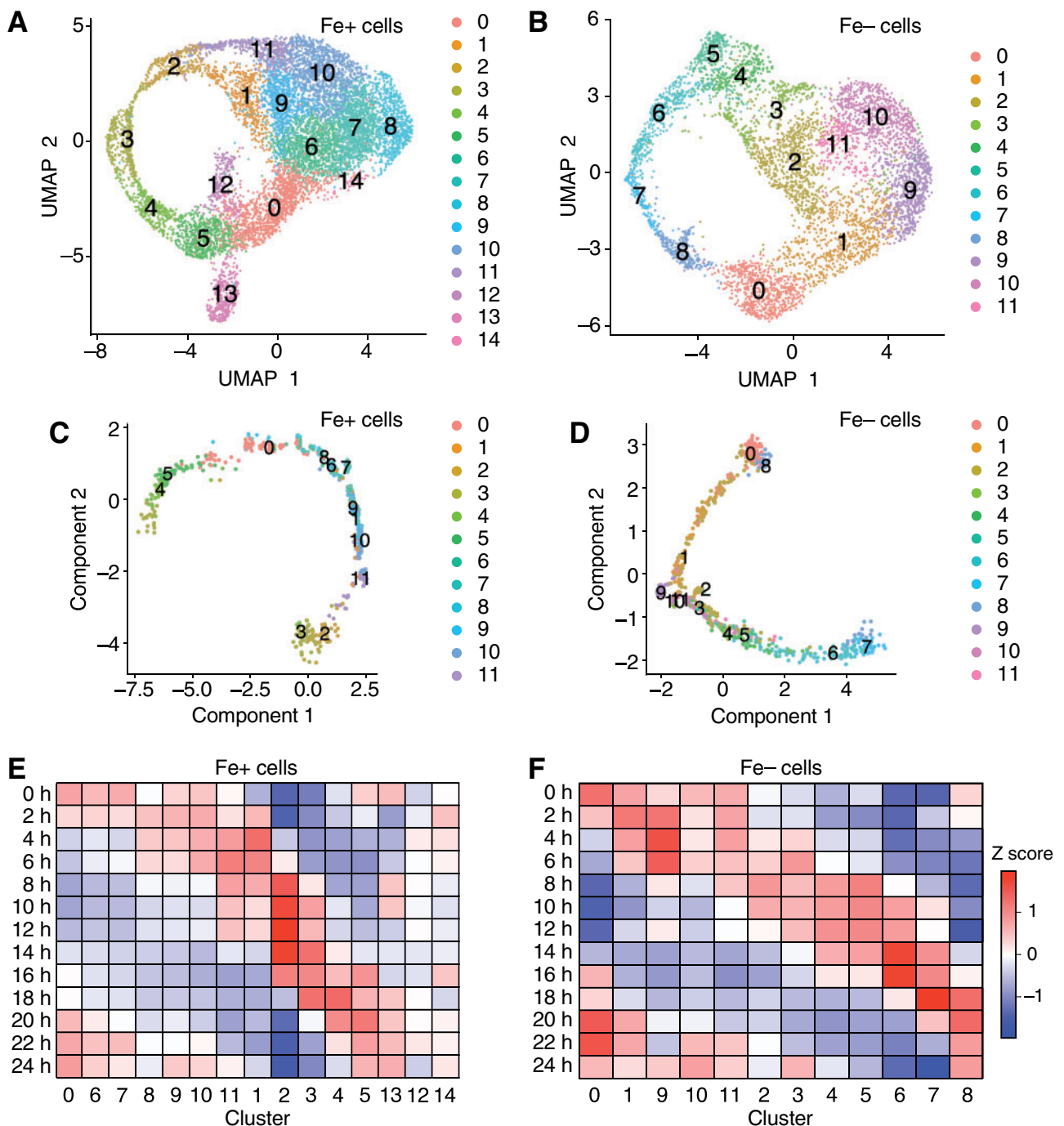
Figure 3. The endogenous diurnal phase of individual cells explains the heterogeneity of batch cell cultures. (A) UMAP plot for the 9,517 sequenced cells grown in Fe+ conditions from Experiment 1. The cells were separated into clusters by Seurat (Stuart et al., 2019) and are indicated by the color gradient, with the color key on the right side of the plot. (B) Same as (A), but with 9,748 sequenced cells grown in Fe- conditions from Experiment 1. (C, D), Trajectory plot of Fe+ (C) and Fe- (D) cells from Experiment 1, colored according to their constituent clusters, as determined by Monocle. (E, F), Heatmap representation of the average diurnal module scores associated with all clusters identified for Fe+ (E) and Fe- (F) cultures. We calculated a diurnal module score for each cluster in 1-h phase bins based on diurnal phase data reported by Zones et al. (2015) of high-confidence rhythmic genes, defined as the overlap of rhythmic genes from two recent studies (Zones et al., 2015; Strenkert et al., 2019).
